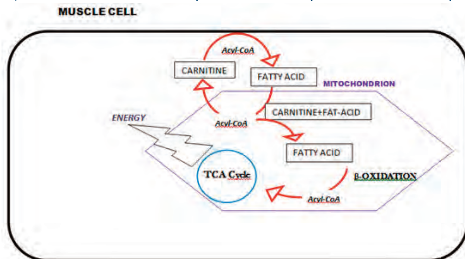
Figure 1: Simplified mechanism of \beta -oxidation during in the muscle cell. The picture shows the importance of carnitine and different acyl-coA enzymes in the transport of fatty-acids into the mitochondria and their contribution to lipid metabolism.
