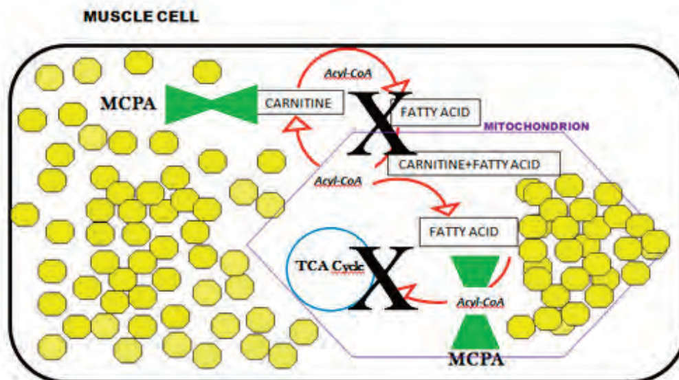
Figure 2. Proposed mechanism of action of MCPA: accumulation of fatty acids (showed in yellow) within the mitochondrion followed by excessive lipid storage in the myocyte (showed in yellow). The impairment of the lipid metabolism leads to myocyte degeneration and Zenker necrosis of the muscle.
